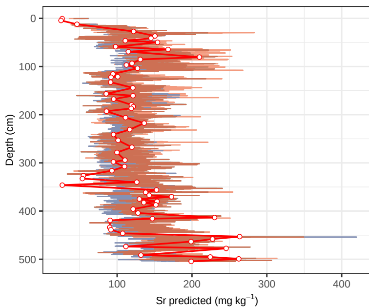
Site BI10 – Sr (depth, multivariate)
